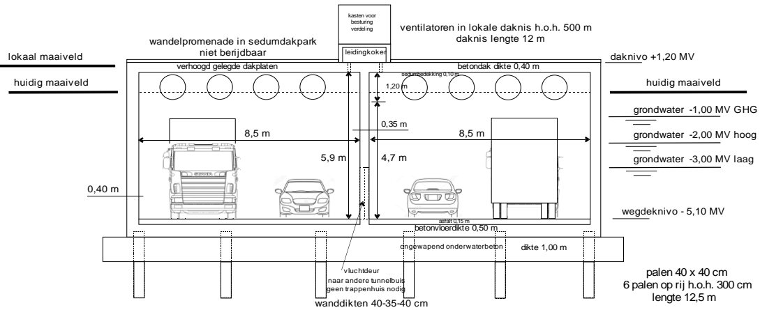
VKA++ tunnelsegment volverdiept
